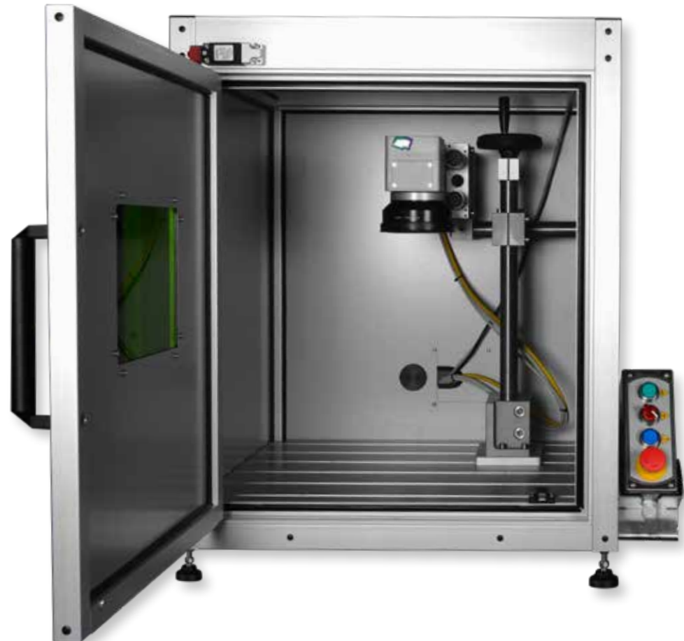
Viewing window and internal LEDs lighting. Vertical position adjustment for marking from above; it comes with handwheel and millimetric references
